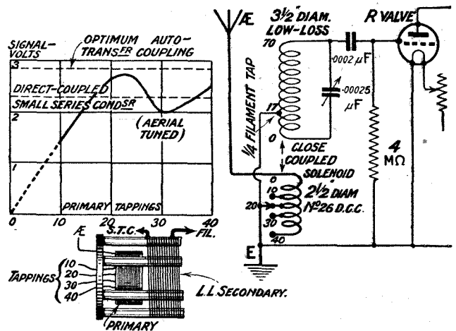
Fig. 4.—When the primary and secondary coupling is tight a peculiar shaped curve results.
